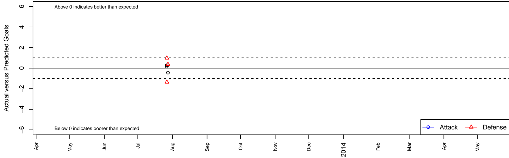
Crossfire Oregon –Unk3 B98 Dots are actual minus expected GF (blue circles) and GA (red triangles). Blue line is smoothed change in attack strength. Red is smoothed change in defense strength.
